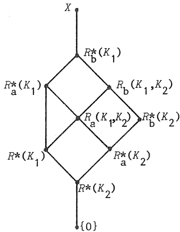
fig. 4.8. Interrelations of 'R'-spaces.
